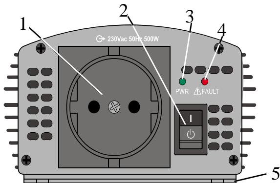
Figure 1 AC Panel on the XPower 500 (European AC Outlet)
