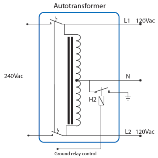
Autotransformer: schematic diagram
