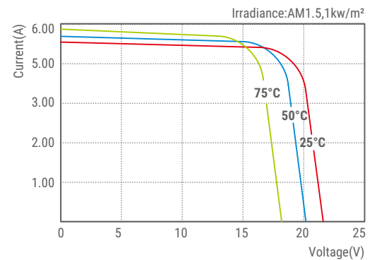
SLP090-24U I-V Curves
