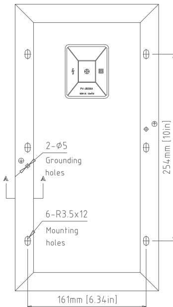
Junction Box Top View (Lid Open)
