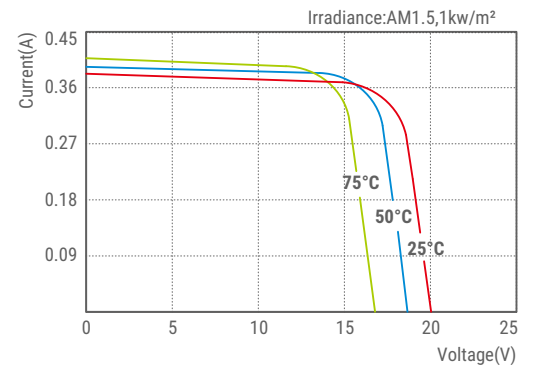
SLP005S-12U I-V Curves
