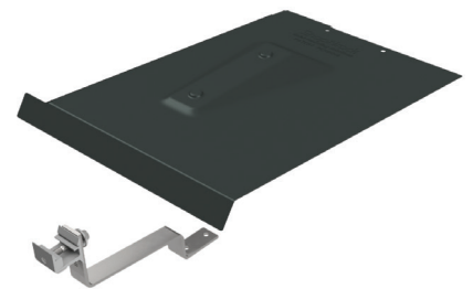
Tile Roof Hook F & Flat Tile Hook Replacement Flashing 242-01247 & 232-60055
