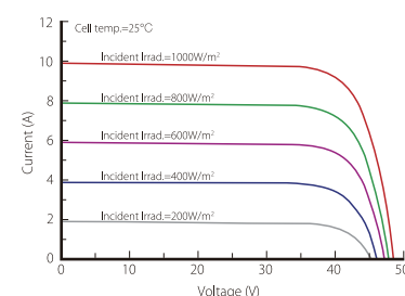
Current-Voltage Curve (LR6-72HIBD-370M)
