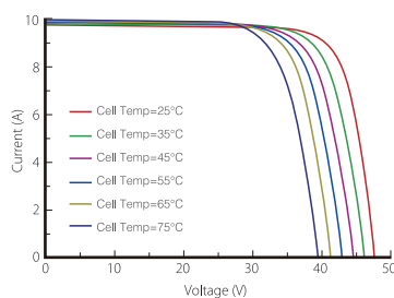
Current-Voltage Curve (LR6-72HIBD-370M)
