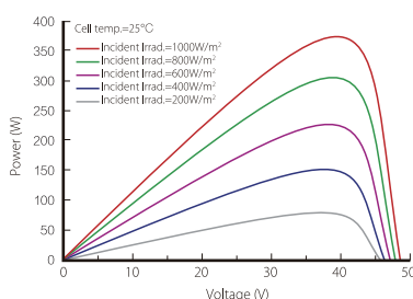
Power-Voltage Curve (LR6-72HIBD-370M)
