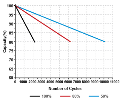
Different DOD Discharge Cycle Life Curve
