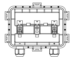
Junction Box Top View (Lid Open)
