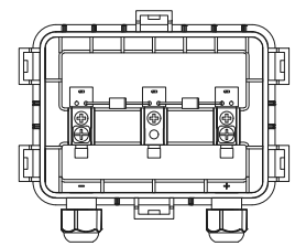
Junction Box Top View (Lid Open)
