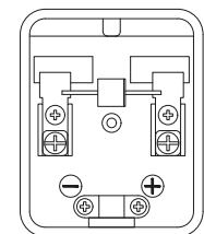
Junction Box Top View (Lid Open)
