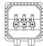
Junction Box Top View (Lid Open)
