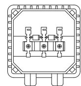
Junction Box Top View (Lid Open)
