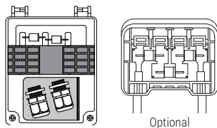
Junction Box Top View (Lid Open)
