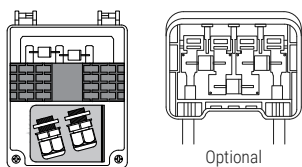
Junction Box Top View (Lid Open)
