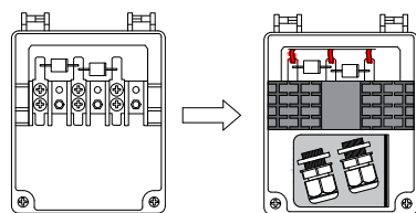
Junction Box Top View (Lid Open)
