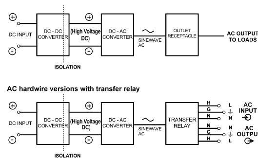
Figure 5. Principles of Operation
