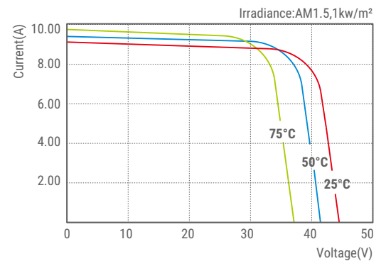
SLP330-24C1D2 I-V Curves
