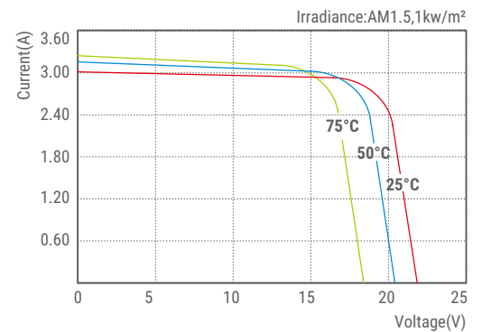
SLP050-12C1D2 I-V Curves
