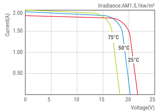
SLP030-12C I-V Curves
