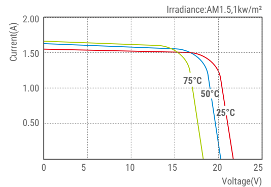
SLP025-12C I-V Curves
