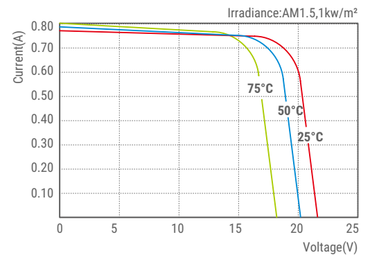
SLP012-12C1D2 I-V Curves
