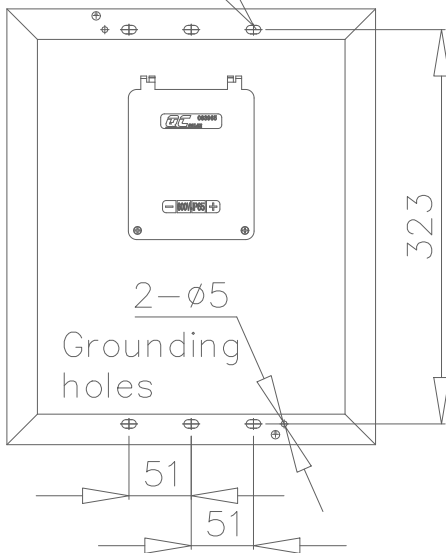
Junction Box Top View (Lid Open)
