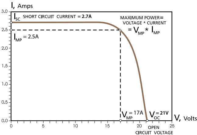
Fig. 2.2. Example of I-V Curve and Ratings of a 12V PV I Solar Panel
