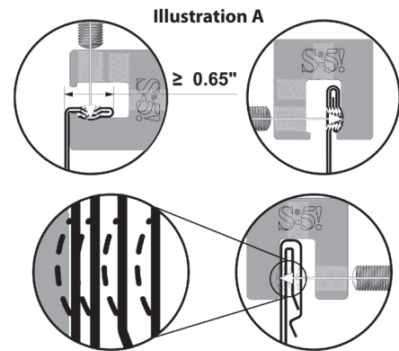
(Top) S-5-U clamp on both vertical and horizontal seams. (Bottom) S-5-S on a snap together seam with blow up illustrating deformation of seam as setscrew is tightened
