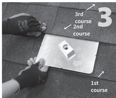
3 Insert flashing between 1st and 2nd course. Slide up so top edge of flashing is at least 3/4" higher than the butt-edge of the 3rd course and lower flashing edge is above the butt-edge of 1st course. Mark center for drilling.
