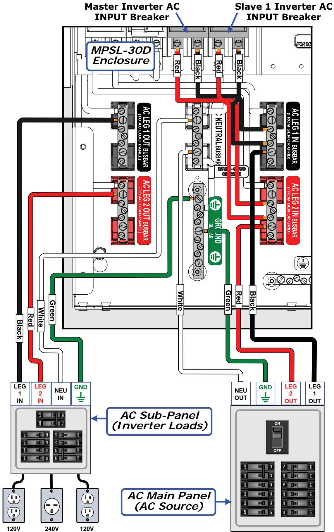
Figure 3-18b, MPXS-30D / MPLS-30D External AC Wiring
