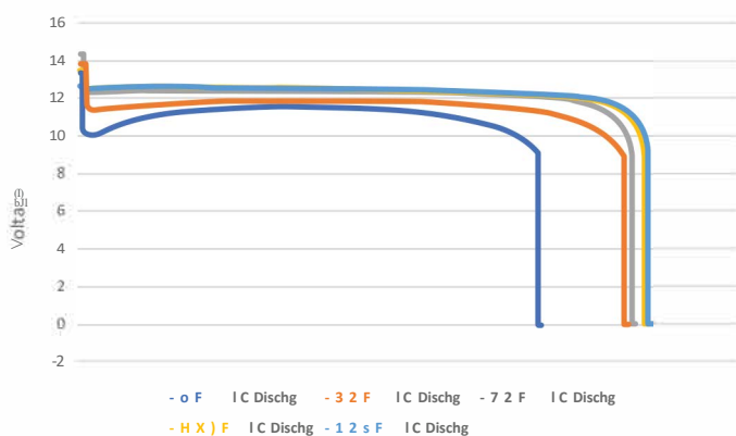
IC Discharge Voltage with Temperature Variations
