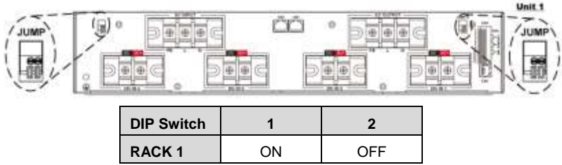
Figure 17-1. Parallel Connection via jumper setting
