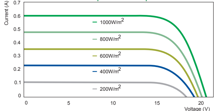
Irradiance - dependence of performance
