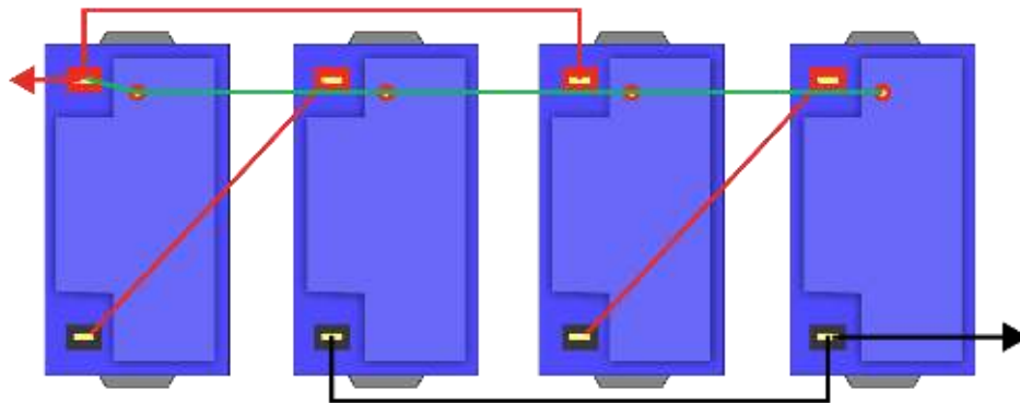
Figure 15: Heat-Enable daisy chained in 24V series/parallel
